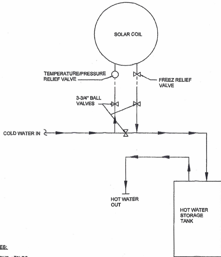
TANK TYPE WATER HEATER PIPING DIAGRAM
