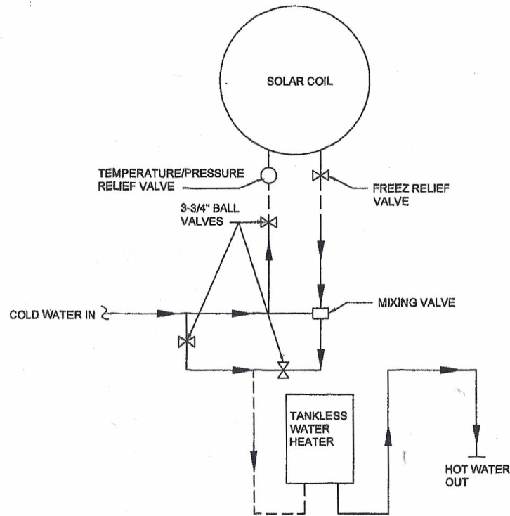
TANKLESS WATER HEATER PIPING DIAGRAM
