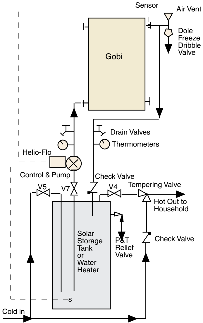
Single Tank System
