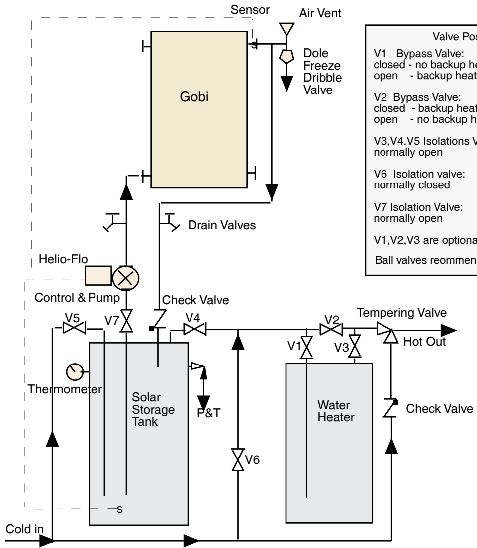
Two Tank System with Separate Backup
