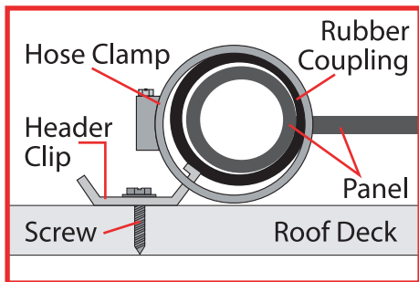
DETAIL A SIDE VIEW
