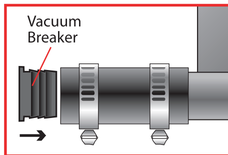
DETAIL C TOP VIEW
